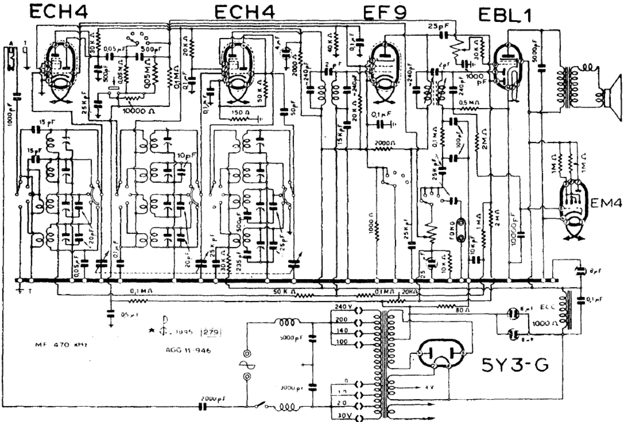
F.I.M.I. - MOD. PHONOLA (583)
